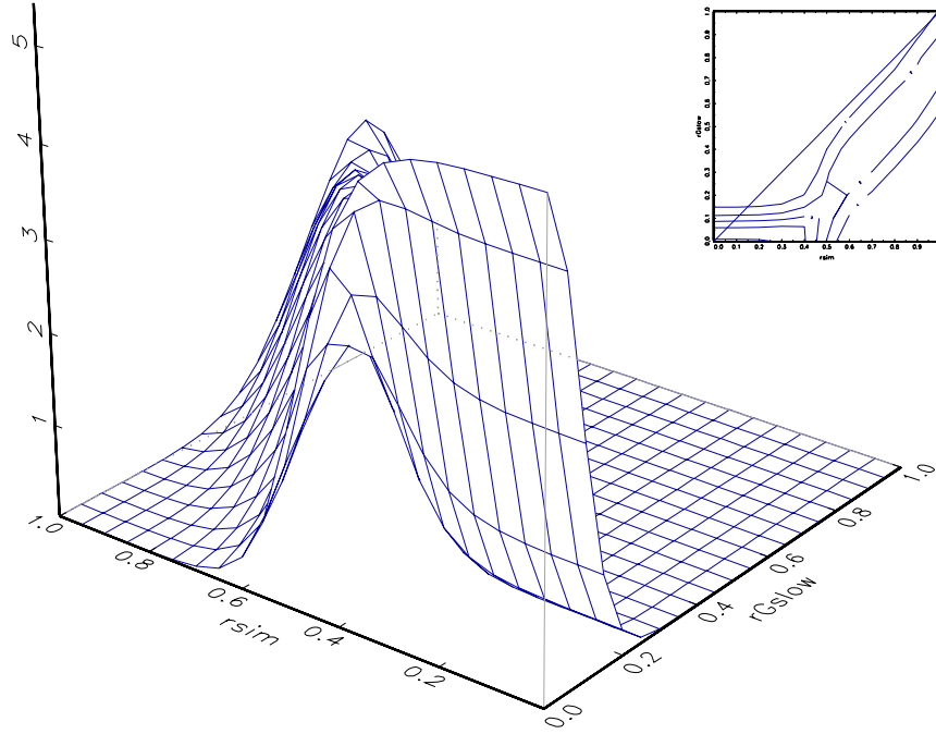
Fig. 8. Stochastic kernel: slow catch-up conditioning
