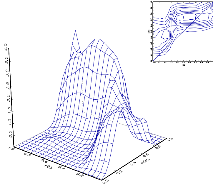
Fig. 4. Stochastic kernel for the distribution in 1995 and the steady-state distribution from model estimates
