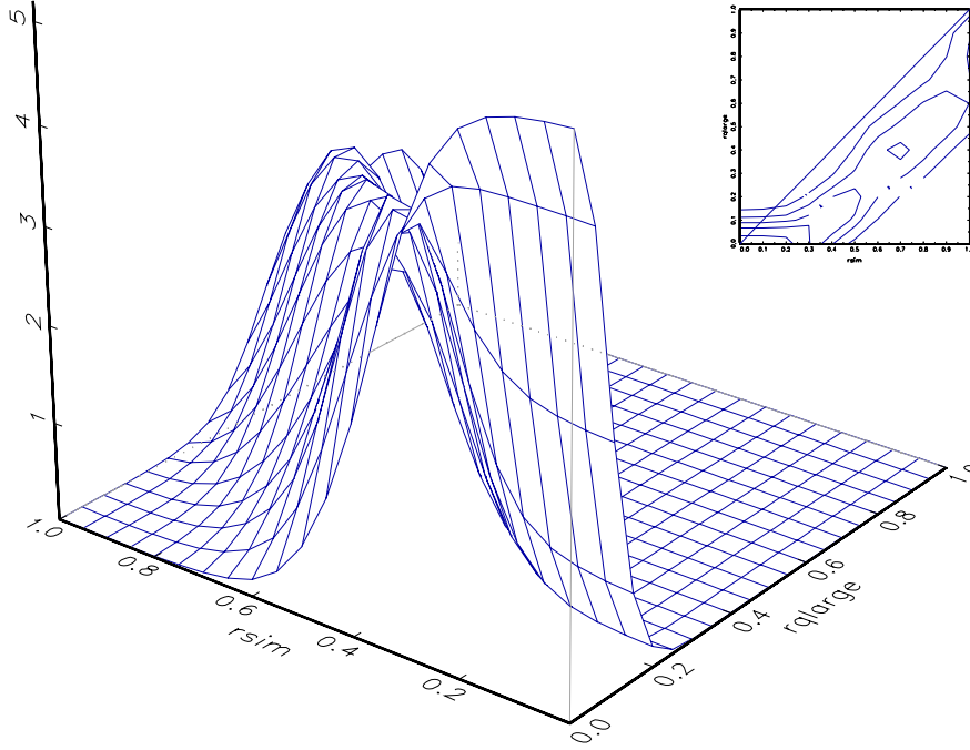
Fig. 10. Stochastic kernel: large RTS conditioning
