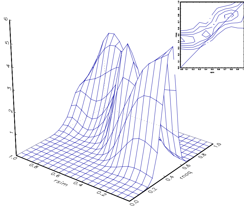
Fig. 5. Stochastic kernel: IRTS conditioning
