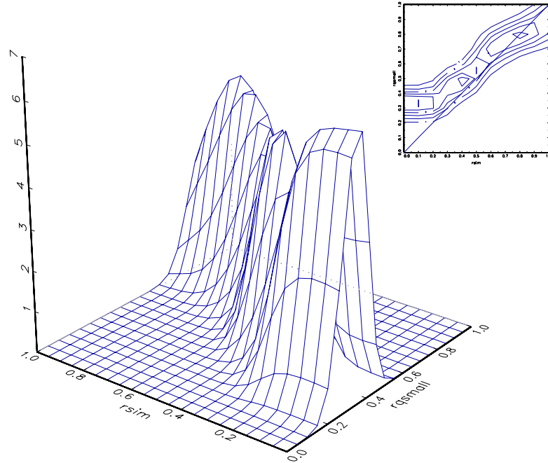
Fig. 9. Stochastic kernel: small RTS conditioning
