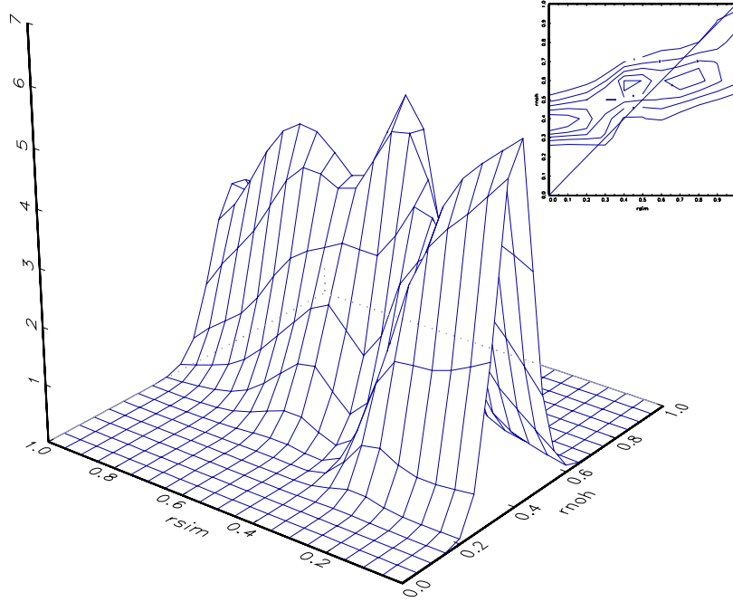
Fig. 6. Stochastic kernel: human capital conditioning
