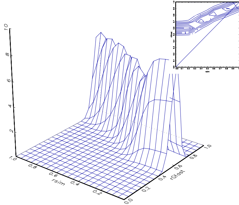
Fig. 7. Stochastic kernel: fast catch-up conditioning
